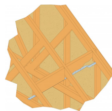
LTS1400E - Lateral Restraint - Fixings to Solid Noggins
