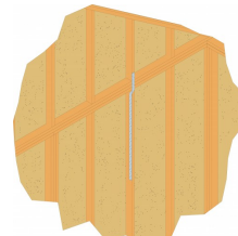
LTS1400E - Vertical Restraint - Timber to Timber Frame
