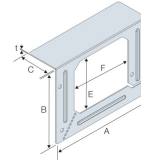
Solid Joist Notch Reinforcement Bracket Dimensions
